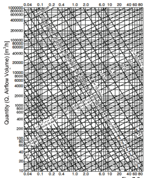
Friction Loss Rate ( \lambda ) [Pa/m] Friction Loss Resistance Chart for Galvanized Steel Pipe
