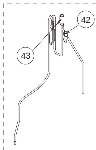
Joint Pipe( injection) Assy
