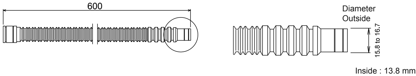
Drain hose
