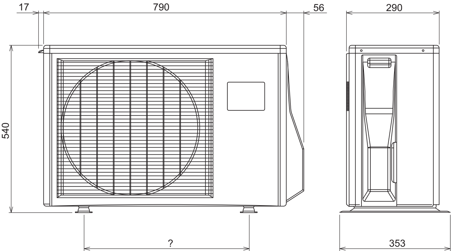
OUTDOOR UNIT
