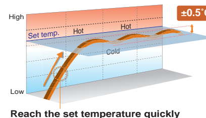
Thermal change of the room *Simulation in heating operation.
