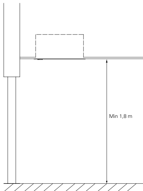
Fig. 4 Minimum distance to the floor for AR200E.
